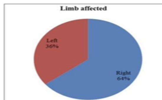
Graph 4: Limb affected
