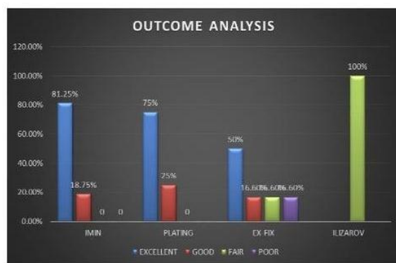
Graph 7: Outcome Analysis
