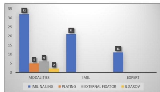
Graph 6: Modalities
