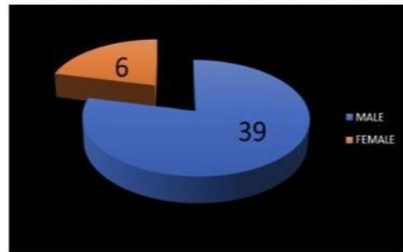
Graph 1: Sex distribution
